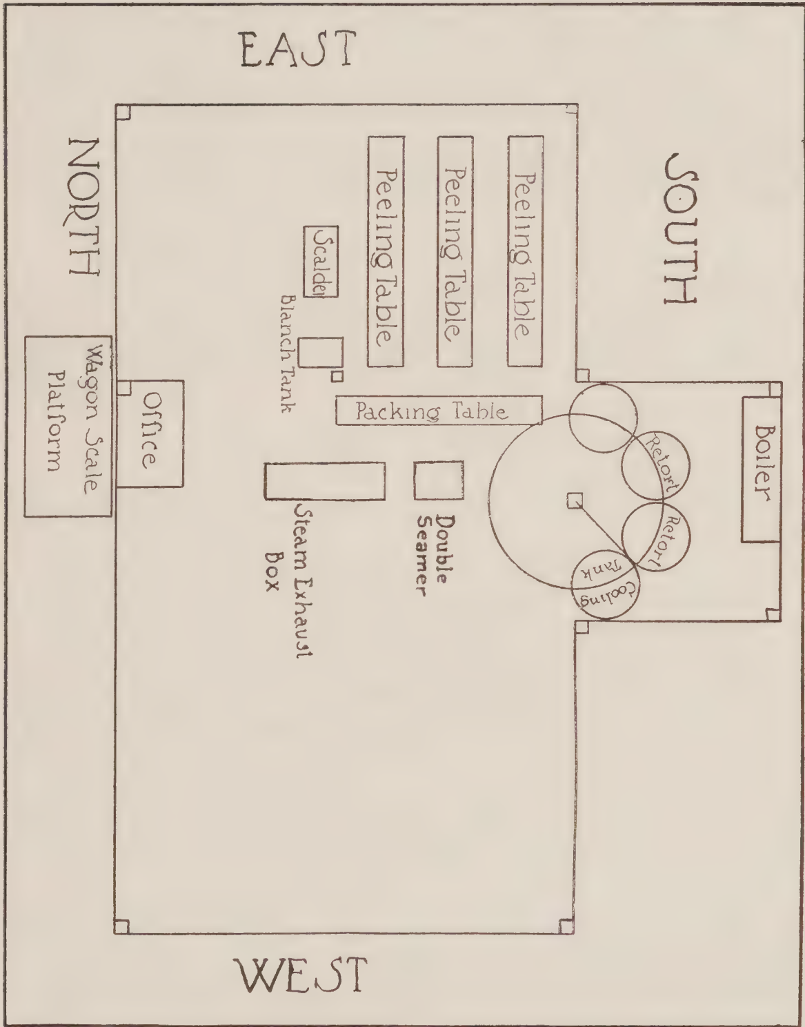
Design of Model Hand-Packing Plant.
